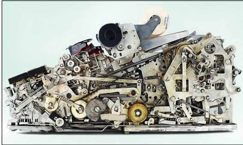
The Monroe mechanical calculator, built in 1964
